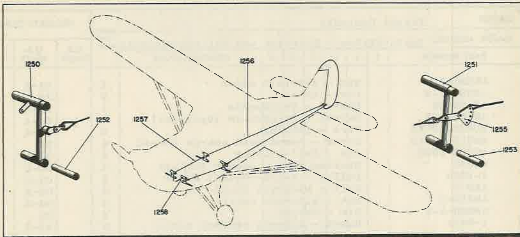
Figure 23 - Rudder Control L-3B & L-3C.
