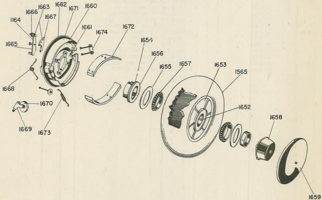
Figure 29 - Van Sickle Wheel & Brake L-3B & L-3C.
