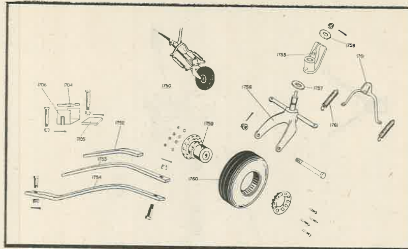
Figure 31 - Steerable Tail Wheel L-3B & L-3C.
