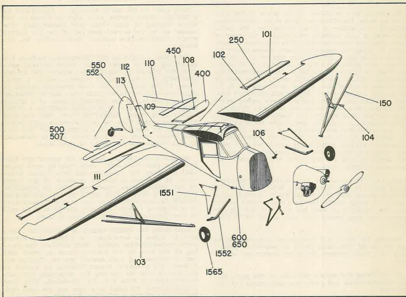
Figure 1 - Major Component Assemblies L-3B & L-3C.
