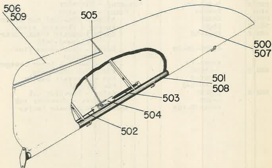
Figure 9 - Left Elevator L-3B & L-3C.
