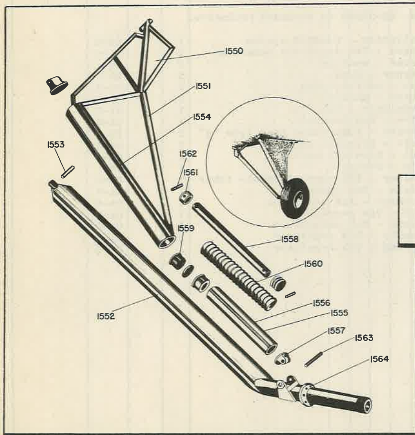
Figure 27 Oleo & Axle Strut O-3B & L-3C.
