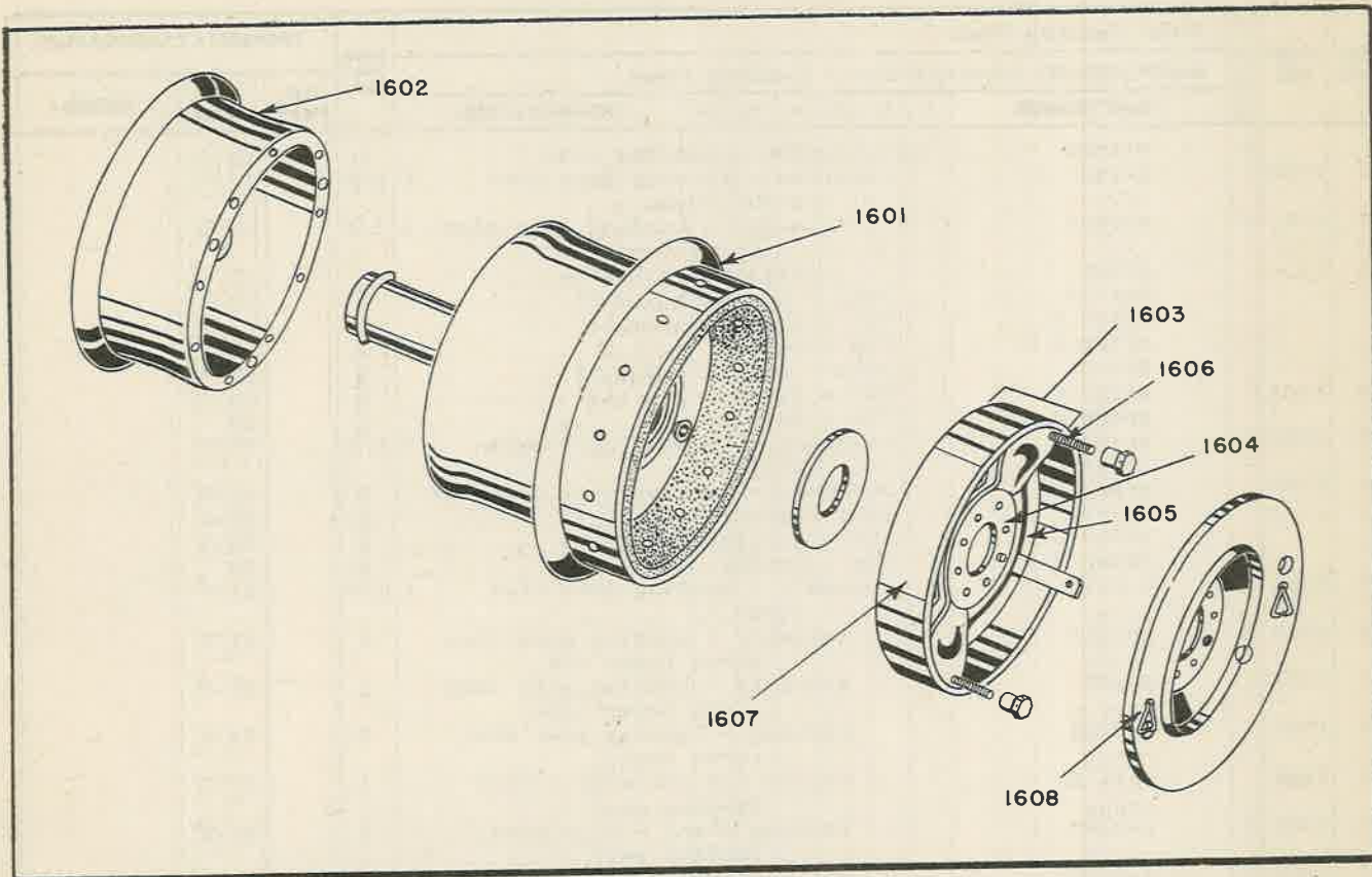
Figure 28 - Shinn Wheel & Brake L-3B & L-3C
