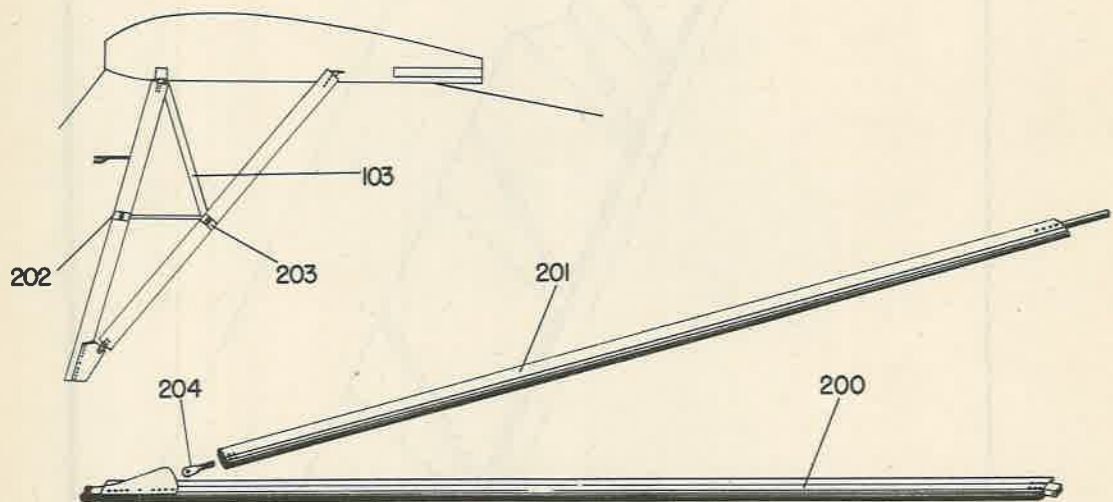
Figure 2 - Steel Struts L-3C.
