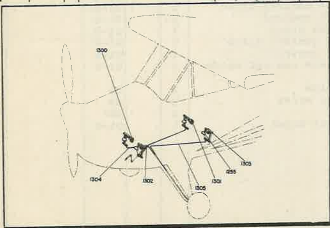
Figure 24 - Dual Brake Control L-3B & L-3C.
