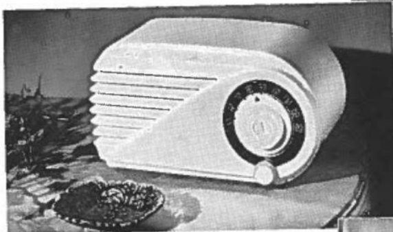
Model GT-050 Smartly styled table radio. Ideal for children's room, Mother's kitchen or Dad's den. Built-in antenna. Automatic volume control. Alnico speaker. Distinctive airplane-type dial for easy, accurate tuning.
